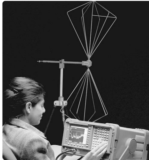
A number of antennas are available with the 84115EM system to test for RF emissions. The E7400 EMC analyzer will also work with other third party antennas.
